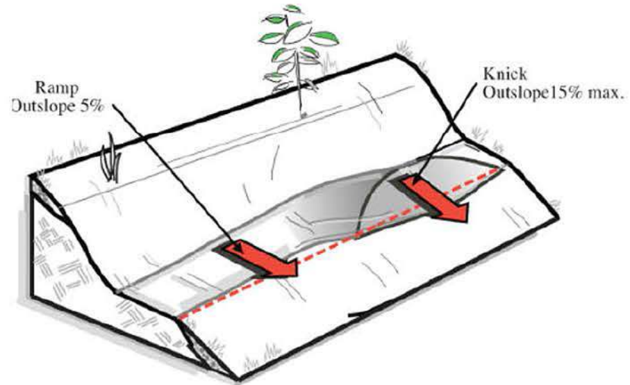
Rolling Grade Dip
